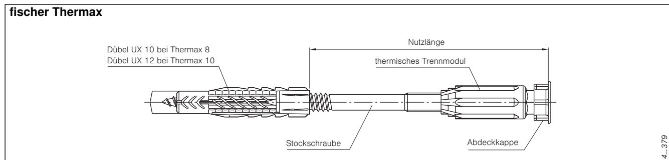
Abb. 282: fischer Thermax
