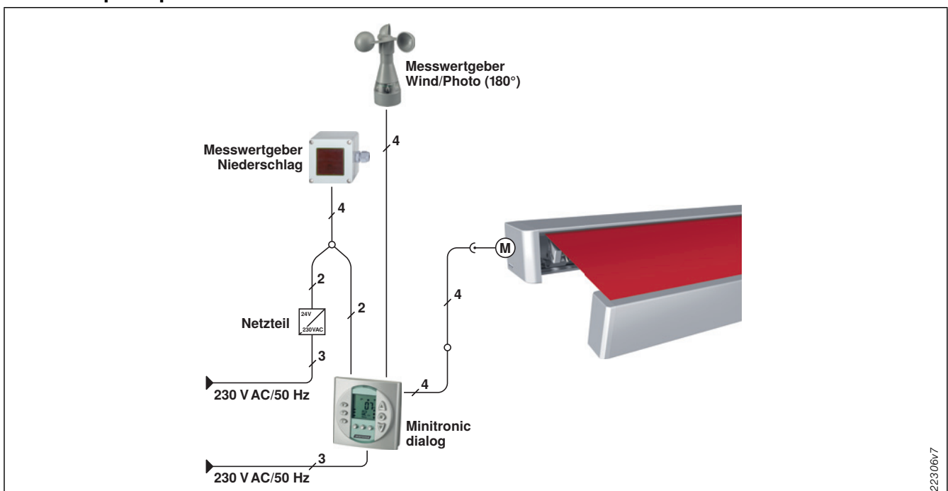
Abb. 293: Minitronic dialog
