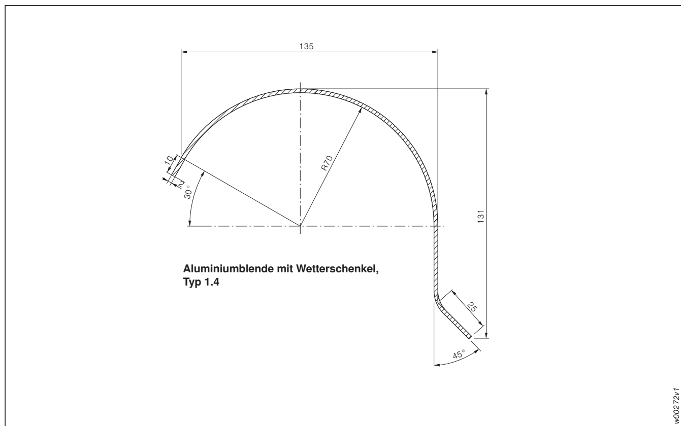
Abb. 150: Aluminium-Blende
